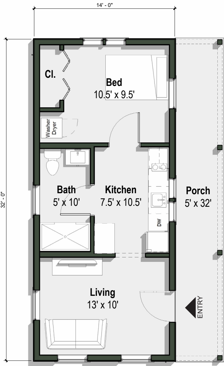
Ground Floor Plan Option III
