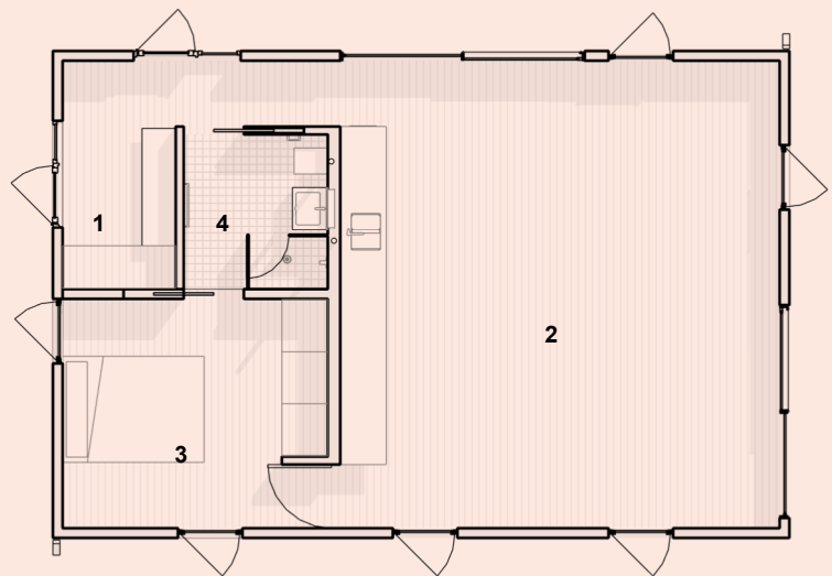
Plan Option 1: Open studio
