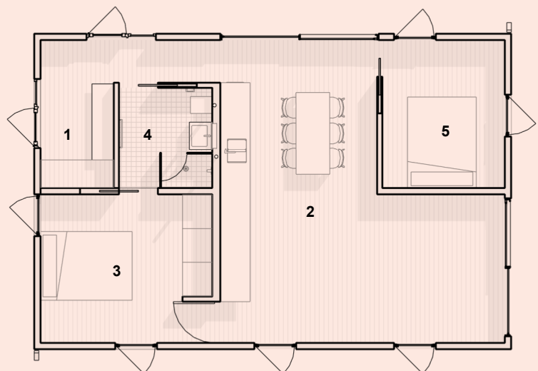
Plan Option 2: 2-bedroom
