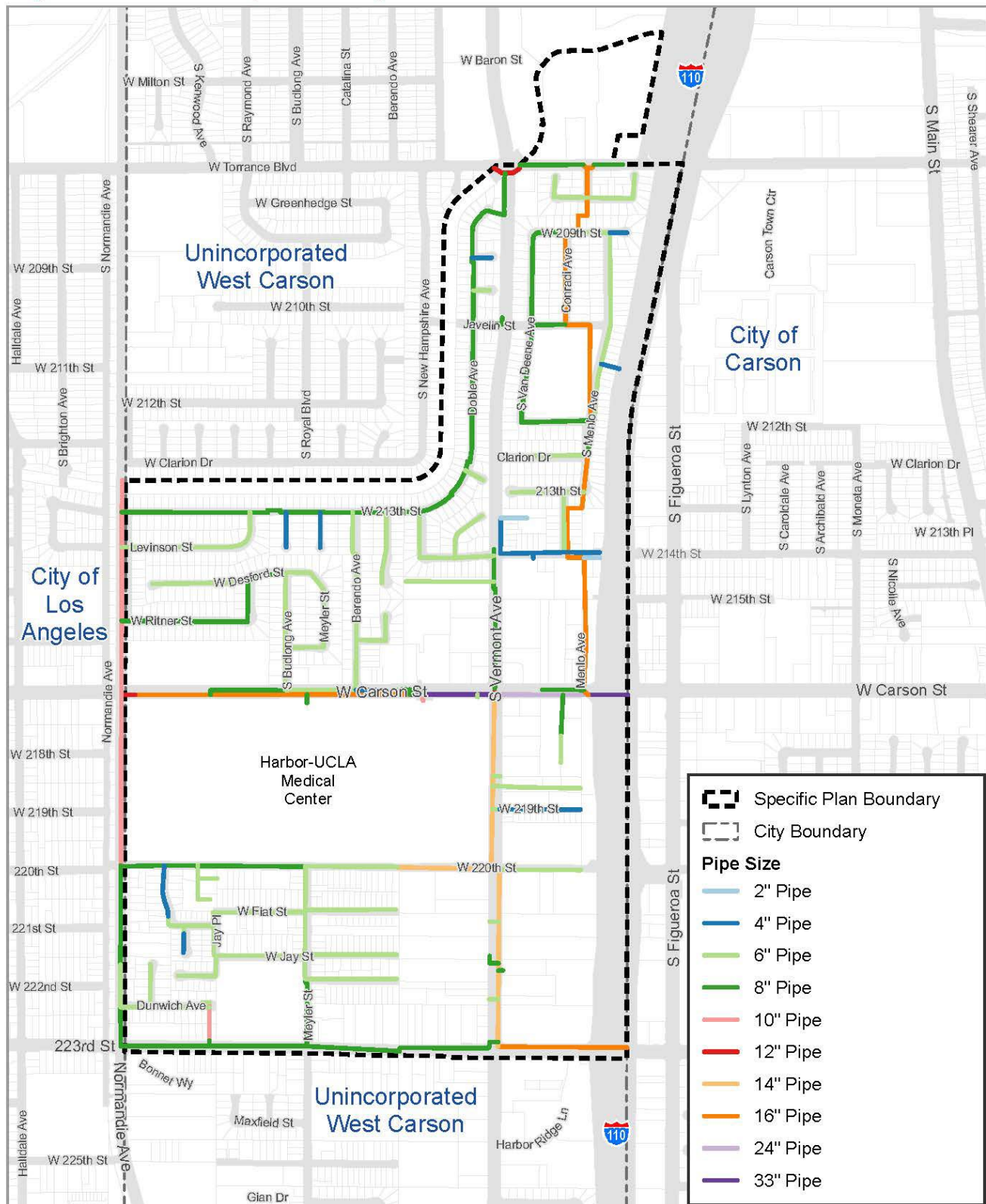
Figure 4-2 Water System - Pipe Size
