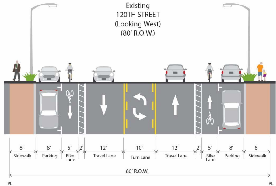
FIGURE 6.16: EXISTING 120TH AVENUE STREETSCAPE
