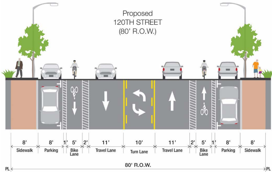
FIGURE 6.17: PROPOSED 120TH STREET STREETSCAPE IMPROVEMENTS
